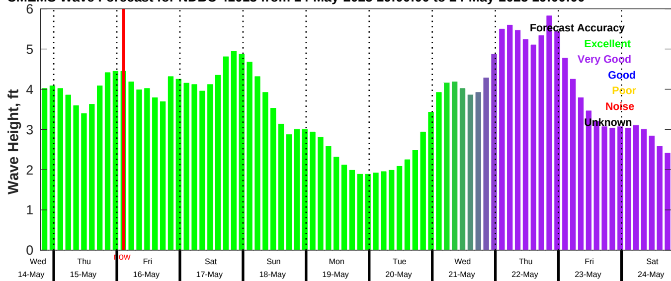
CMEMS Wave Forecast for NDBC 41013 from 14-May-2025 19:00:00 to 24-May-2025 19:00:00
