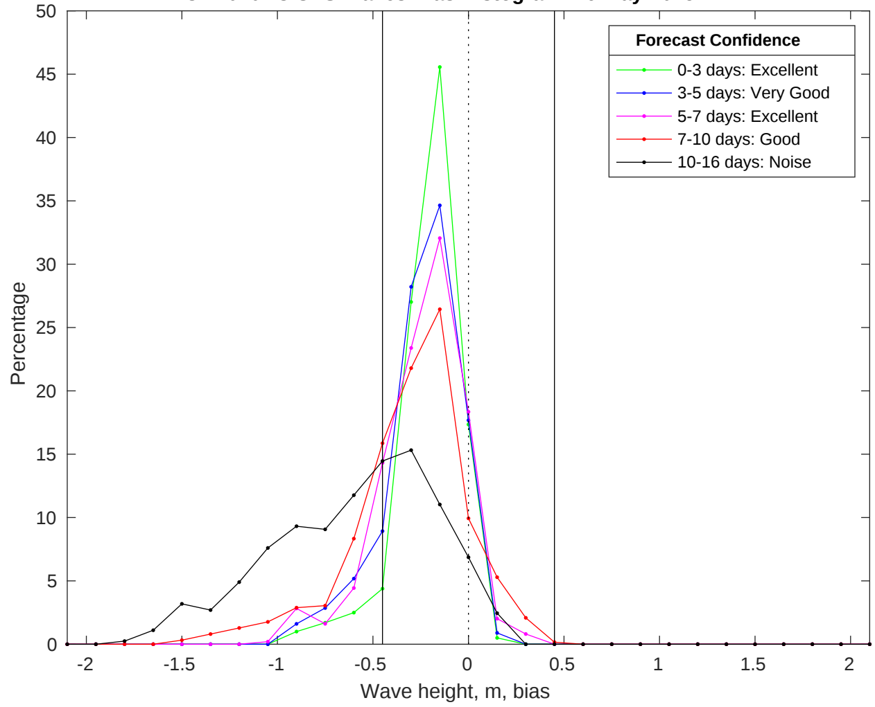
NDBC 41040 vs GFS Waves Bias Histogram: 16-May-2025
