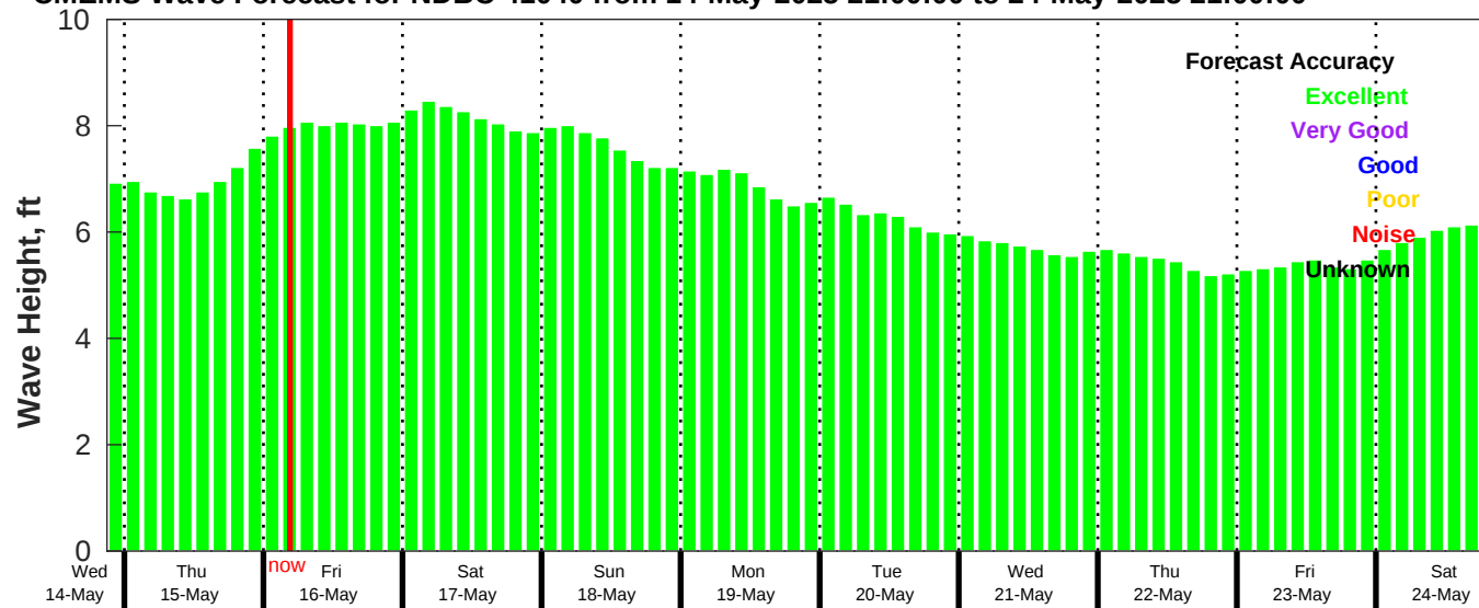
CMEMS Wave Forecast for NDBC 41040 from 14-May-2025 21:00:00 to 24-May-2025 21:00:00
