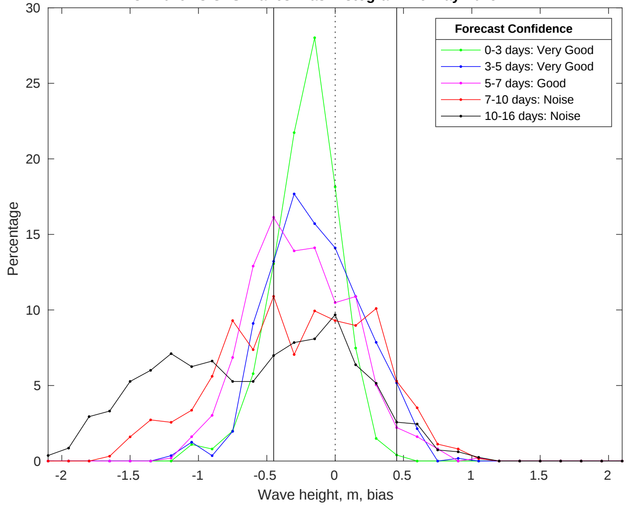
NDBC 42019 vs GFS Waves Bias Histogram: 16-May-2025
