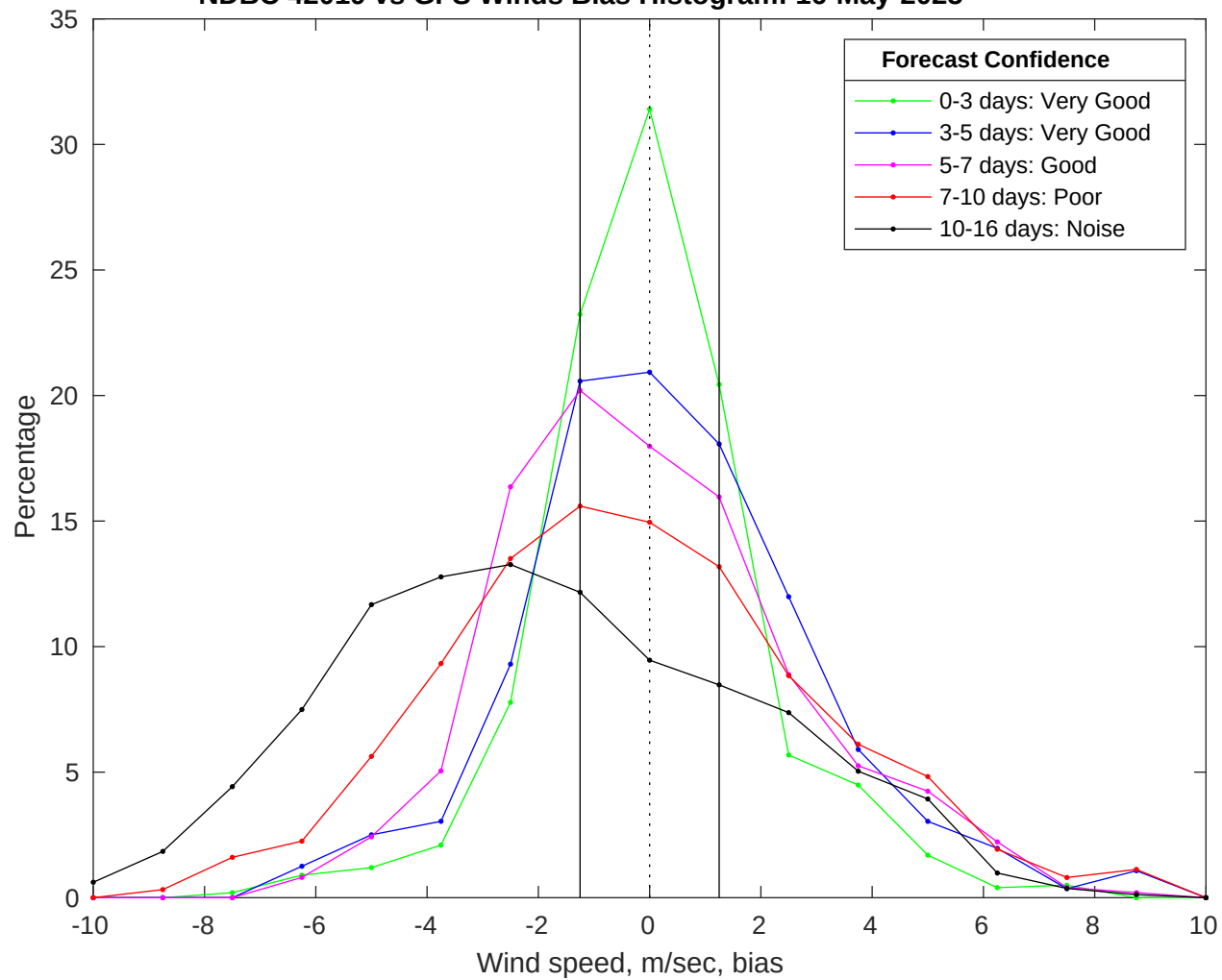
NDBC 42019 vs GFS Winds Bias Histogram: 16-May-2025
