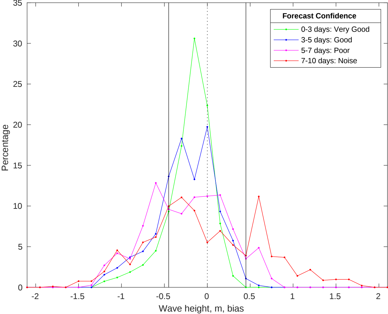
NDBC 42020 vs CMEMS Waves Bias Histogram: 16-May-2025
