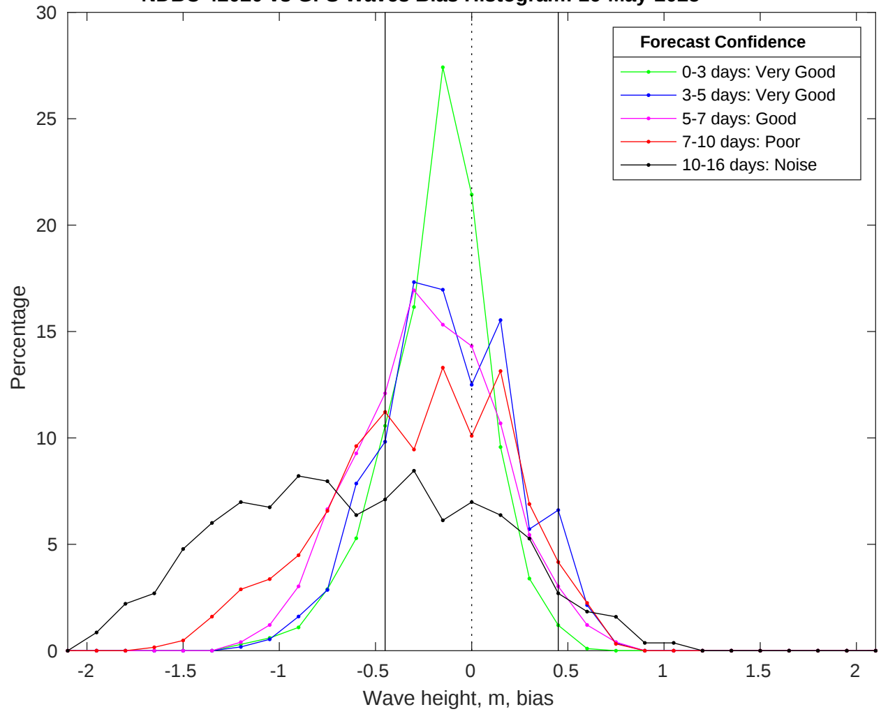
NDBC 42020 vs GFS Waves Bias Histogram: 16-May-2025
