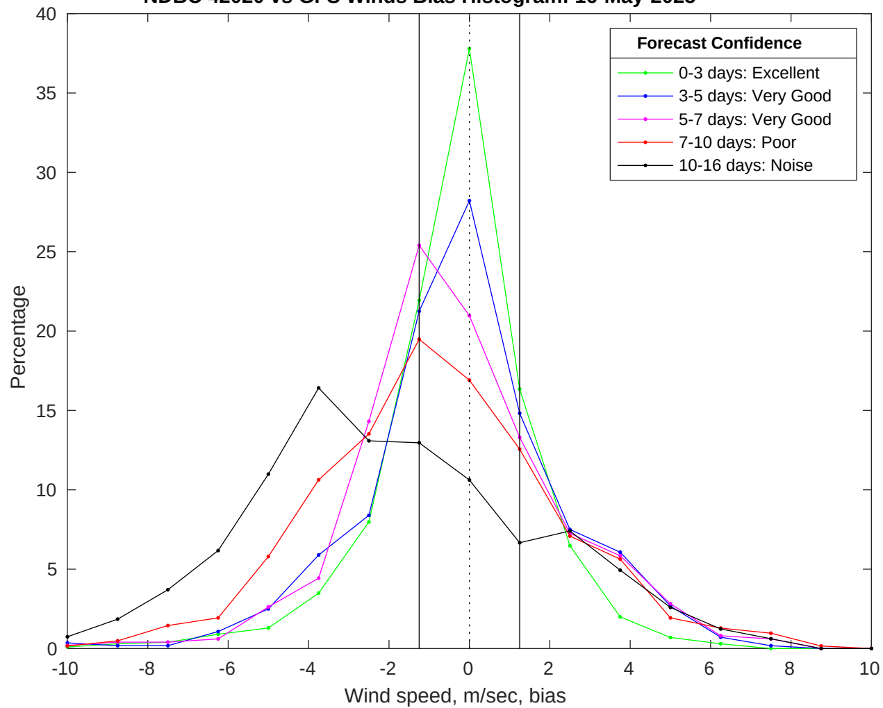
NDBC 42020 vs GFS Winds Bias Histogram: 16-May-2025
