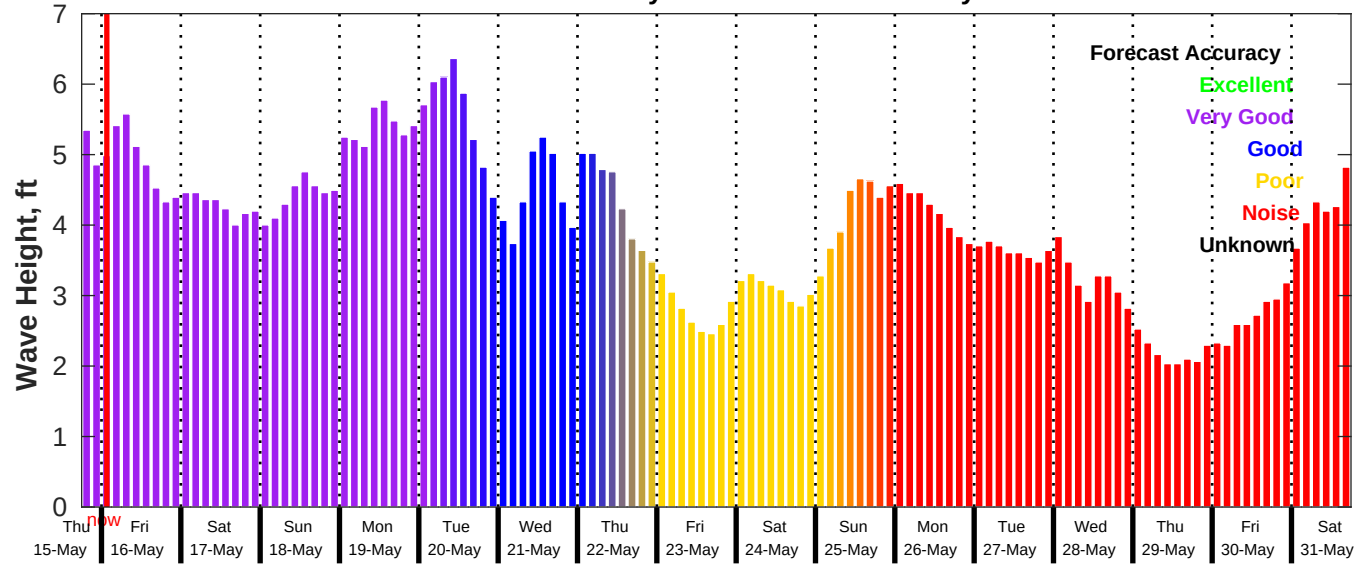
GFS Wave Forecast for NDBC 42020 from 15-May-2025 18:00:00 to 31-May-2025 18:00:00
