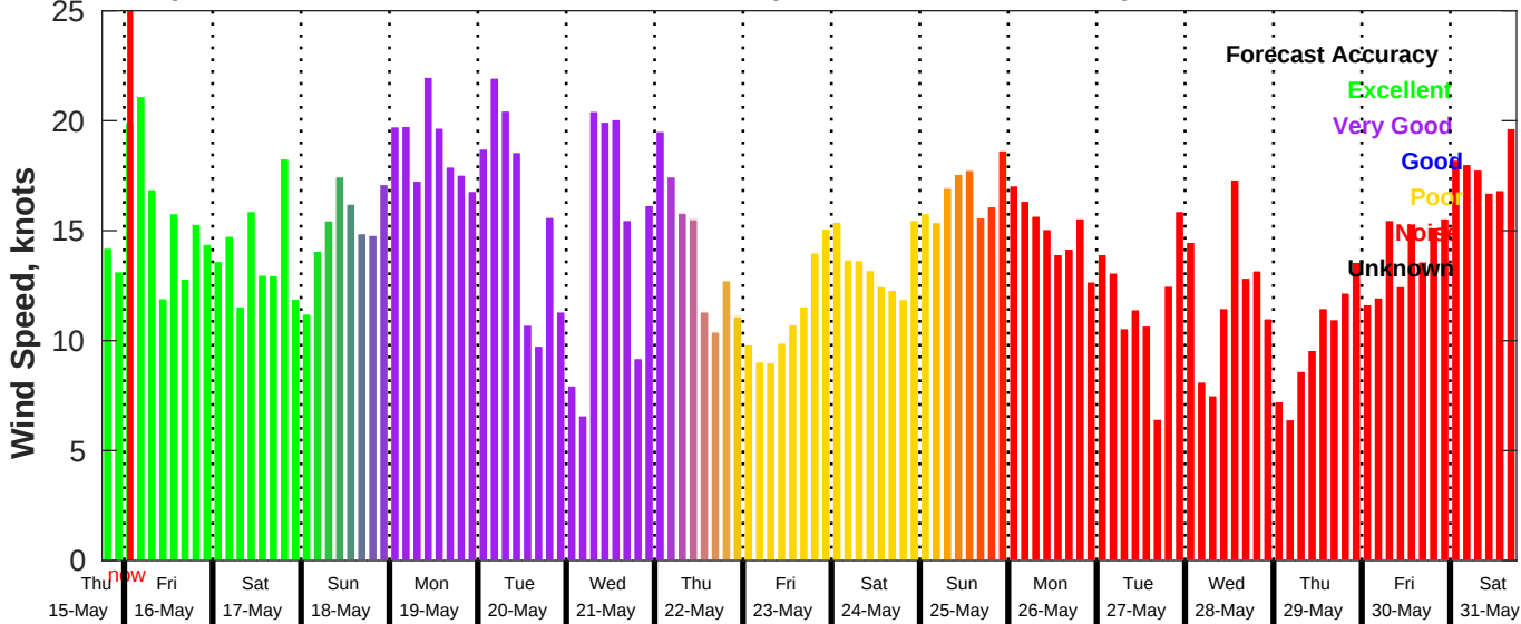
GFS Wind Speed Forecast for NDBC 42020 from 15-May-2025 18:00:00 to 31-May-2025 18:00:00
