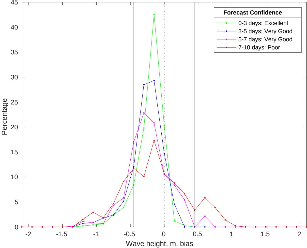
NDBC 42035 vs CMEMS Waves Bias Histogram: 16-May-2025
