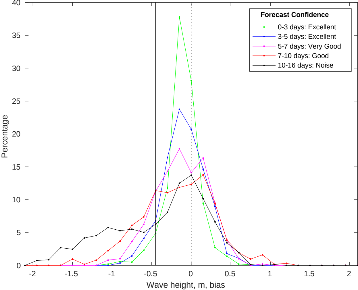
NDBC 42035 vs GFS Waves Bias Histogram: 16-May-2025
