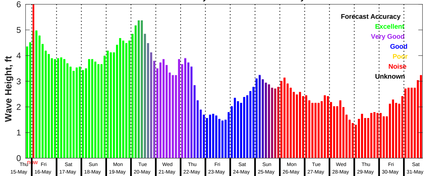
GFS Wave Forecast for NDBC 42035 from 15-May-2025 18:00:00 to 31-May-2025 18:00:00
