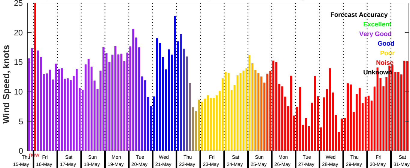
GFS Wind Speed Forecast for NDBC 42035 from 15-May-2025 18:00:00 to 31-May-2025 18:00:00
