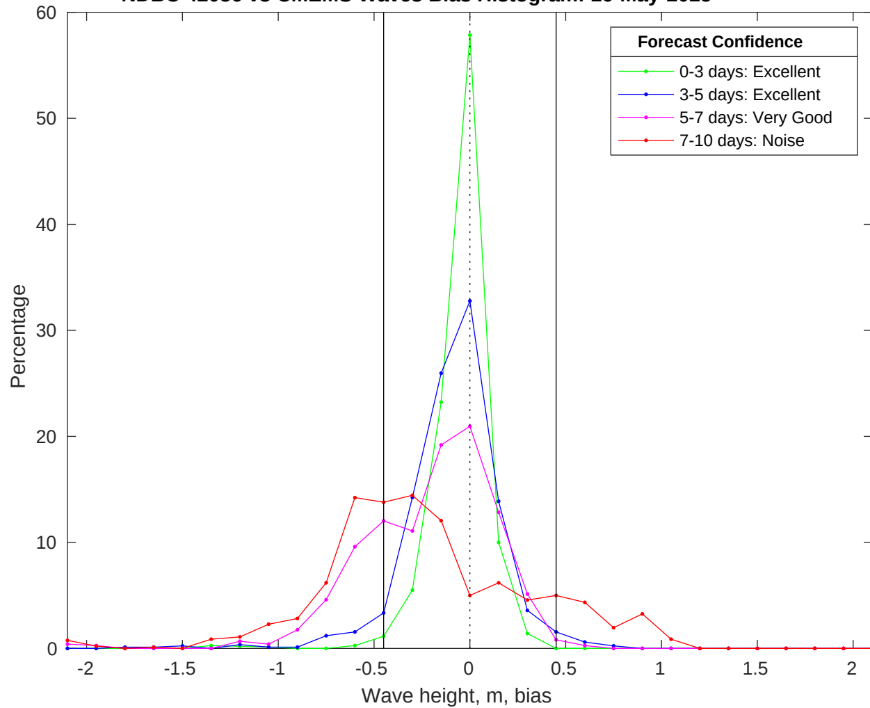
NDBC 42036 vs CMEMS Waves Bias Histogram: 16-May-2025
