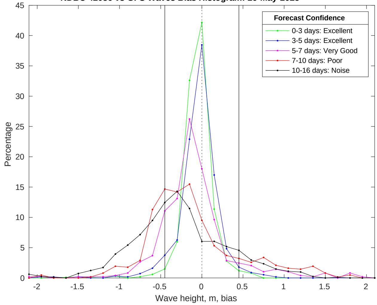
NDBC 42036 vs GFS Waves Bias Histogram: 16-May-2025
