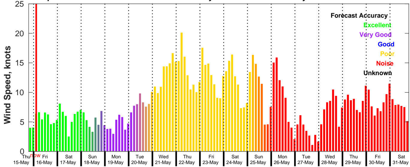
GFS Wind Speed Forecast for NDBC 42036 from 15-May-2025 19:00:00 to 31-May-2025 19:00:00
