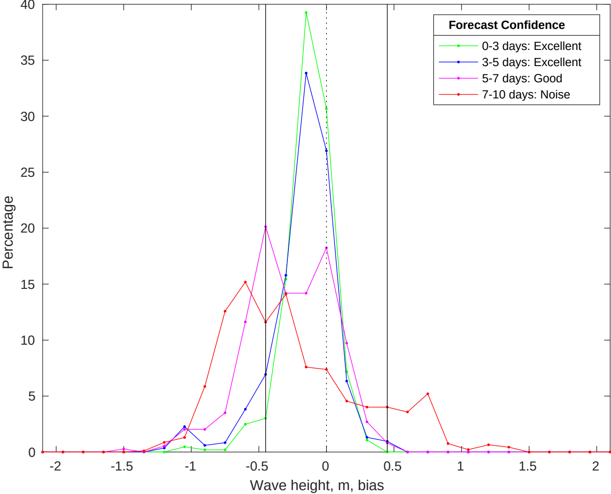
NDBC 42040 vs CMEMS Waves Bias Histogram: 16-May-2025
