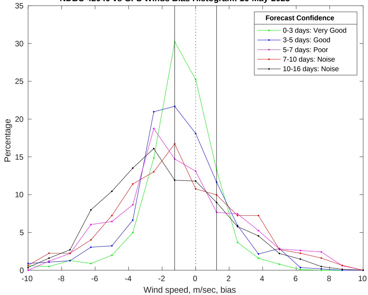
NDBC 42040 vs GFS Winds Bias Histogram: 16-May-2025
