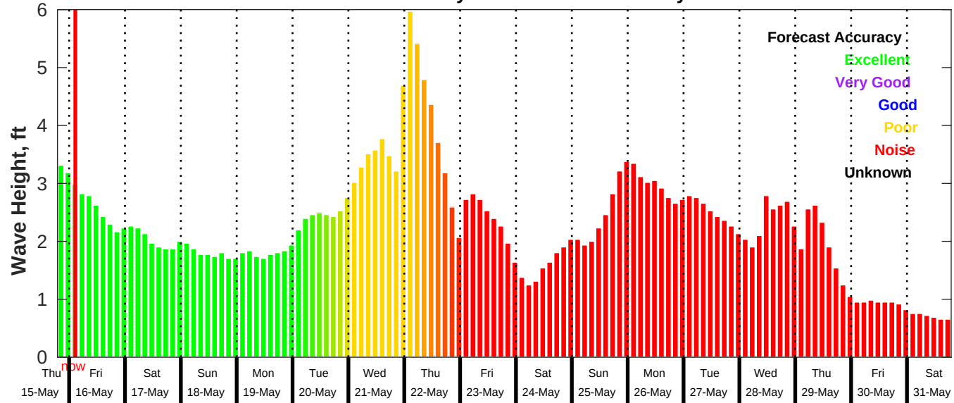
GFS Wave Forecast for NDBC 42040 from 15-May-2025 19:00:00 to 31-May-2025 19:00:00
