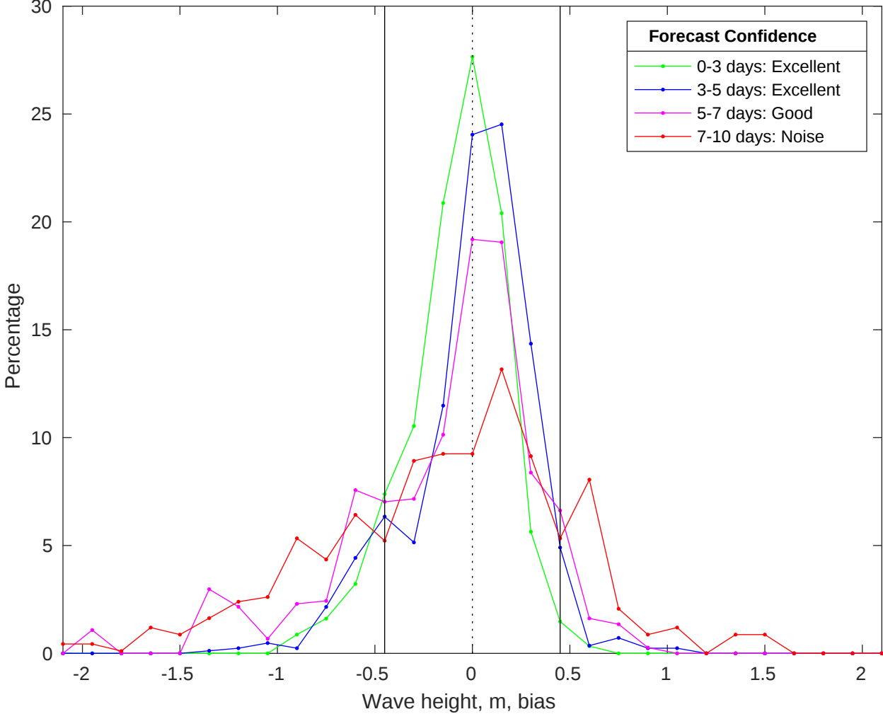
NDBC 46011 vs CMEMS Waves Bias Histogram: 16-May-2025
