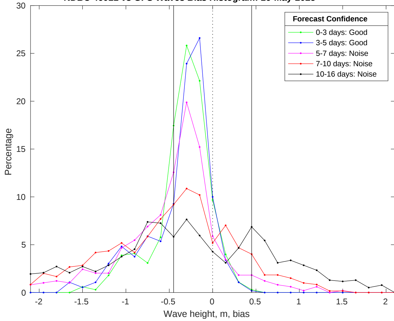
NDBC 46011 vs GFS Waves Bias Histogram: 16-May-2025
