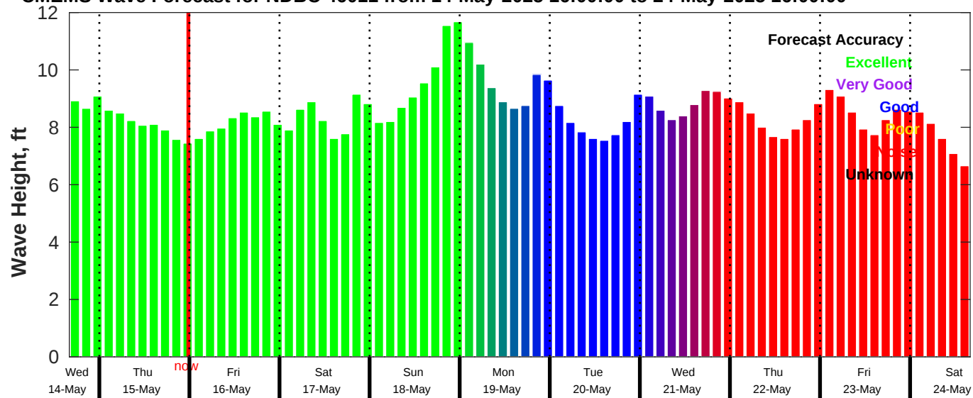
CMEMS Wave Forecast for NDBC 46011 from 14-May-2025 16:00:00 to 24-May-2025 16:00:00
