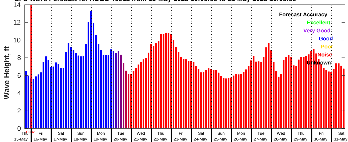
GFS Wave Forecast for NDBC 46011 from 15-May-2025 16:00:00 to 31-May-2025 16:00:00
