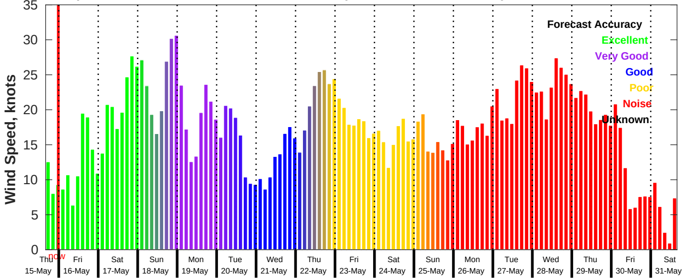
GFS Wind Speed Forecast for NDBC 46011 from 15-May-2025 16:00:00 to 31-May-2025 16:00:00
