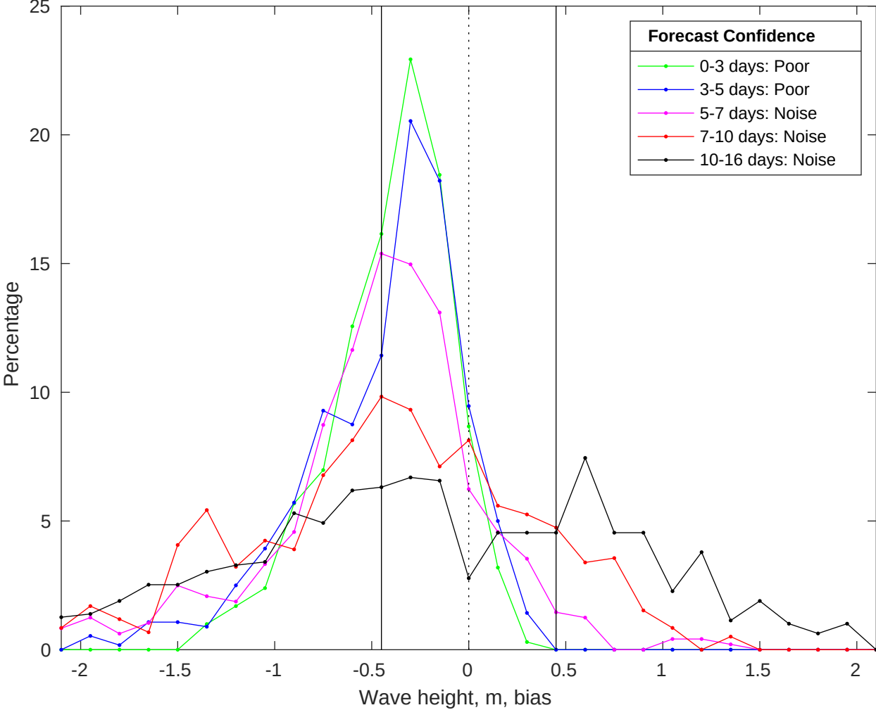
NDBC 46028 vs GFS Waves Bias Histogram: 16-May-2025
