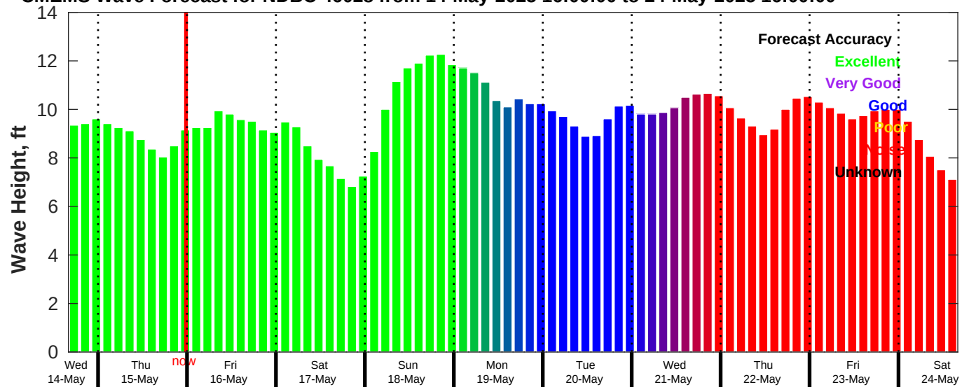
CMEMS Wave Forecast for NDBC 46028 from 14-May-2025 16:00:00 to 24-May-2025 16:00:00
