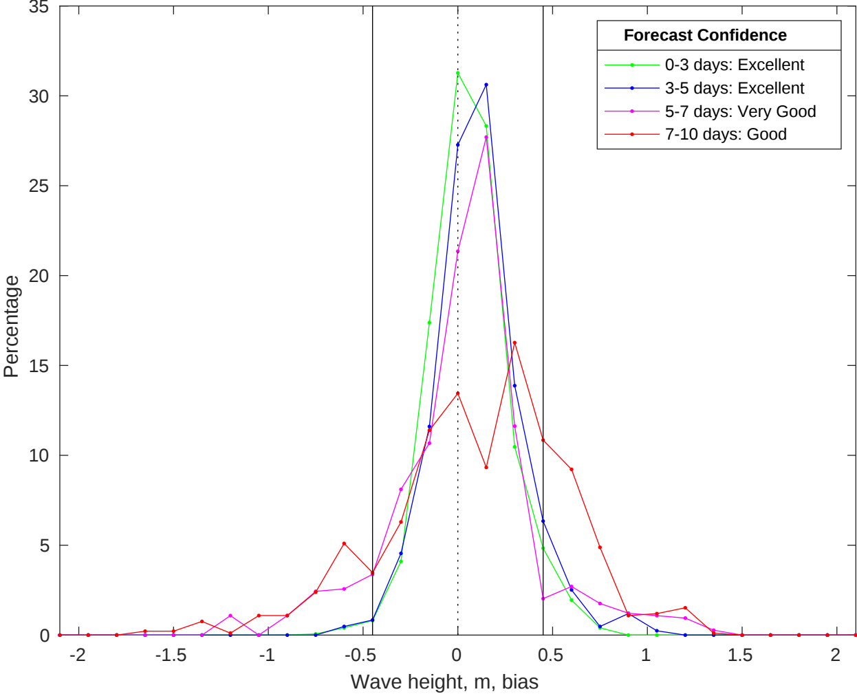
NDBC 46054 vs CMEMS Waves Bias Histogram: 16-May-2025
