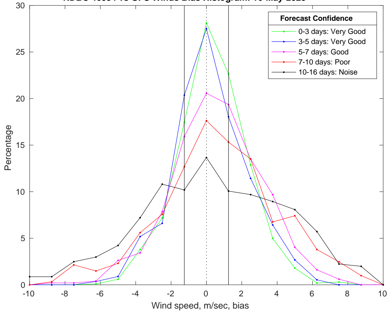
NDBC 46054 vs GFS Winds Bias Histogram: 16-May-2025
