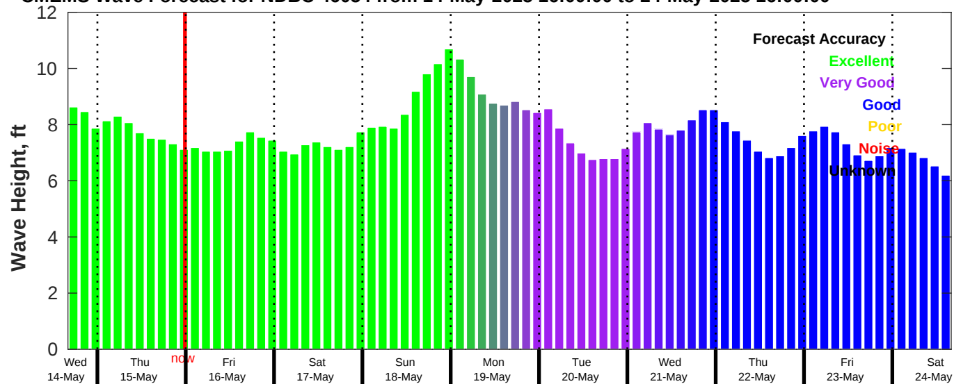
CMEMS Wave Forecast for NDBC 46054 from 14-May-2025 16:00:00 to 24-May-2025 16:00:00
