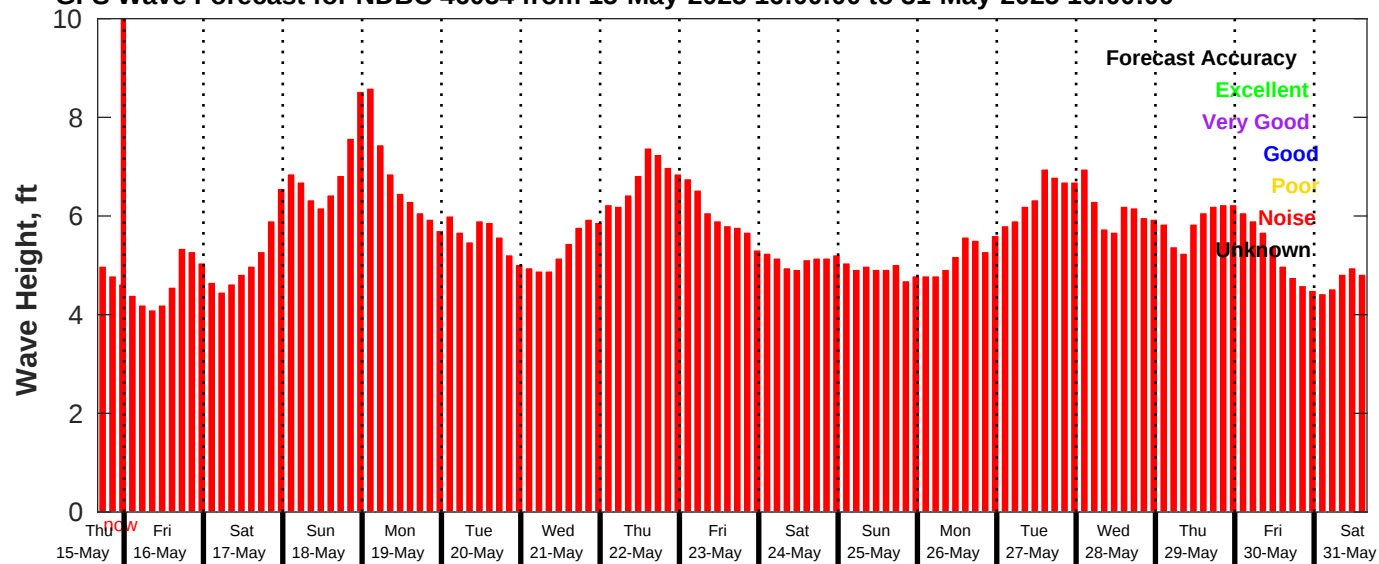
GFS Wave Forecast for NDBC 46054 from 15-May-2025 16:00:00 to 31-May-2025 16:00:00
