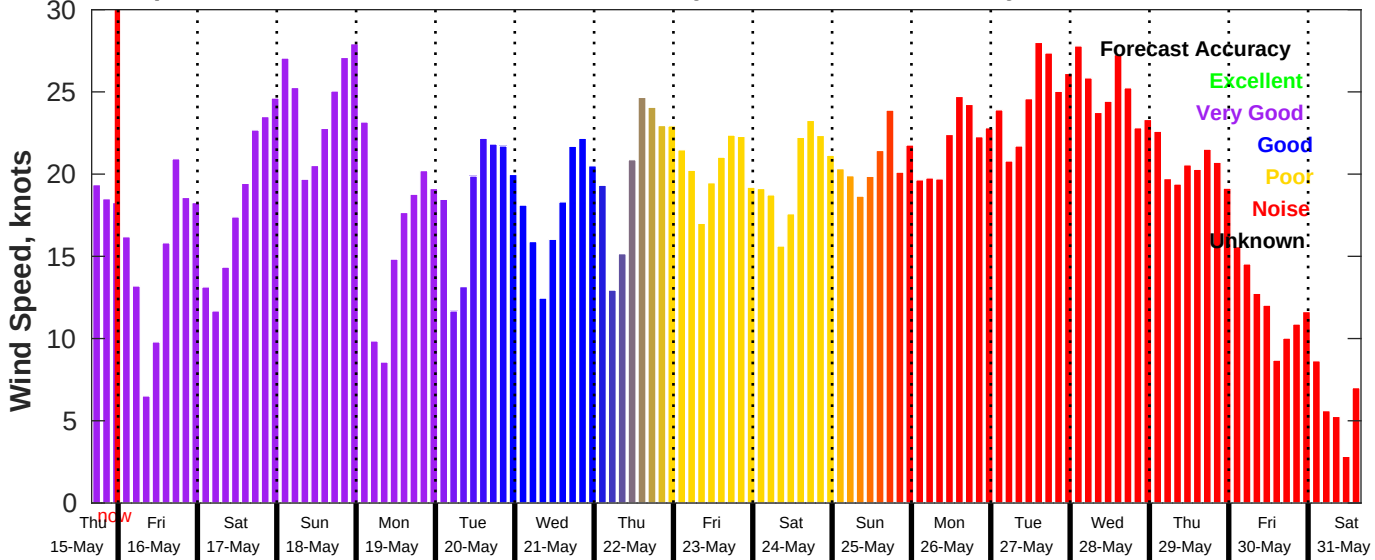
GFS Wind Speed Forecast for NDBC 46054 from 15-May-2025 16:00:00 to 31-May-2025 16:00:00
