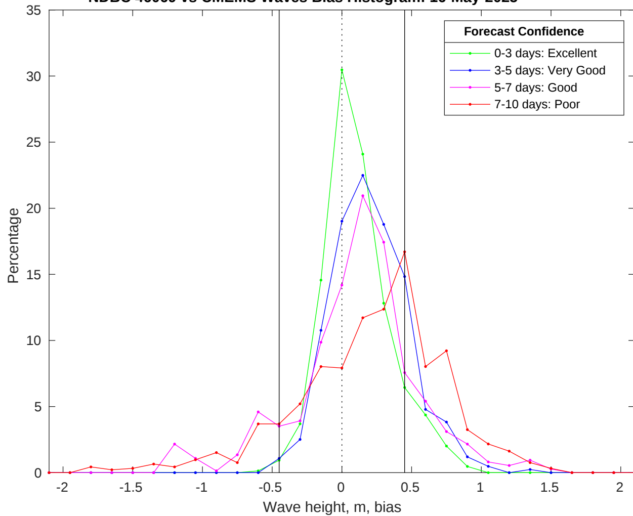
NDBC 46069 vs CMEMS Waves Bias Histogram: 16-May-2025
