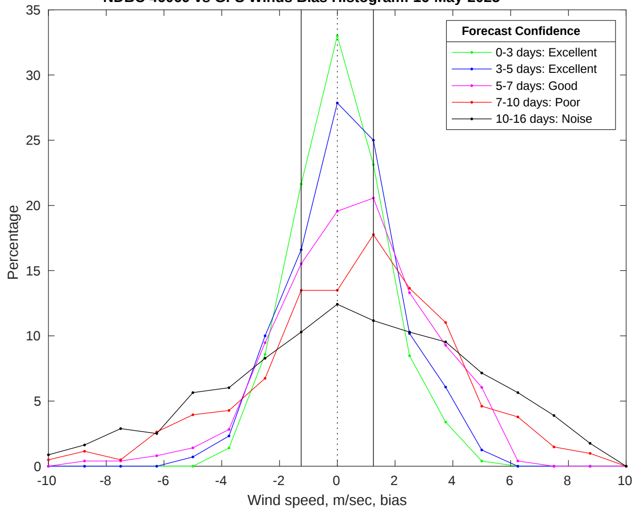
NDBC 46069 vs GFS Winds Bias Histogram: 16-May-2025
