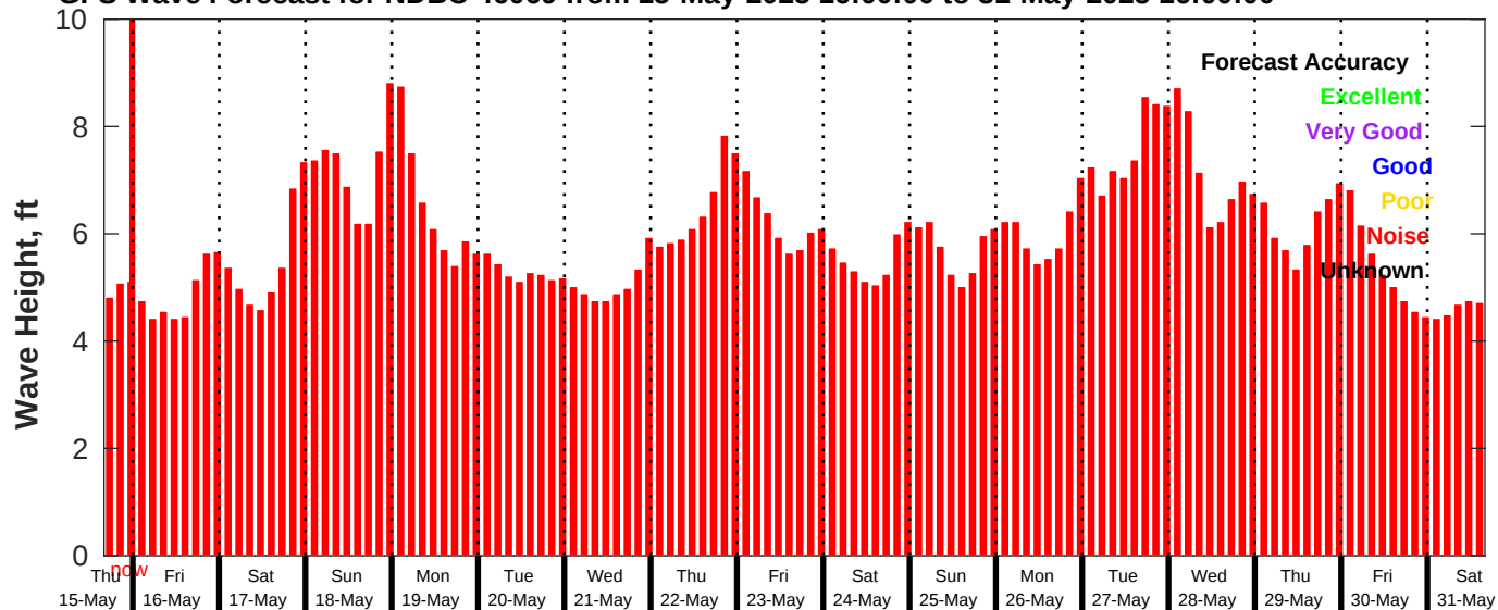
GFS Wave Forecast for NDBC 46069 from 15-May-2025 16:00:00 to 31-May-2025 16:00:00
