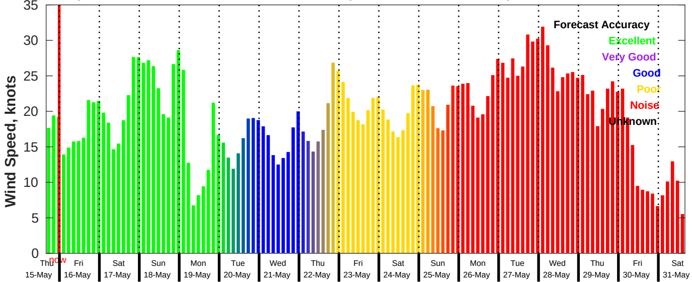
GFS Wind Speed Forecast for NDBC 46069 from 15-May-2025 16:00:00 to 31-May-2025 16:00:00
