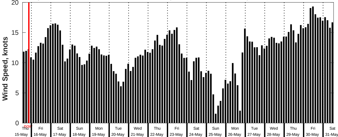
GFS Wind Speed Forecast for NDBC 51209 from 15-May-2025 13:00:00 to 31-May-2025 13:00:00
