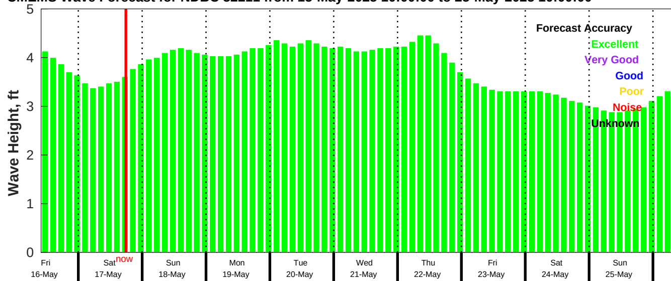
CMEMS Wave Forecast for NDBC 52211 from 15-May-2025 10:00:00 to 25-May-2025 10:00:00
