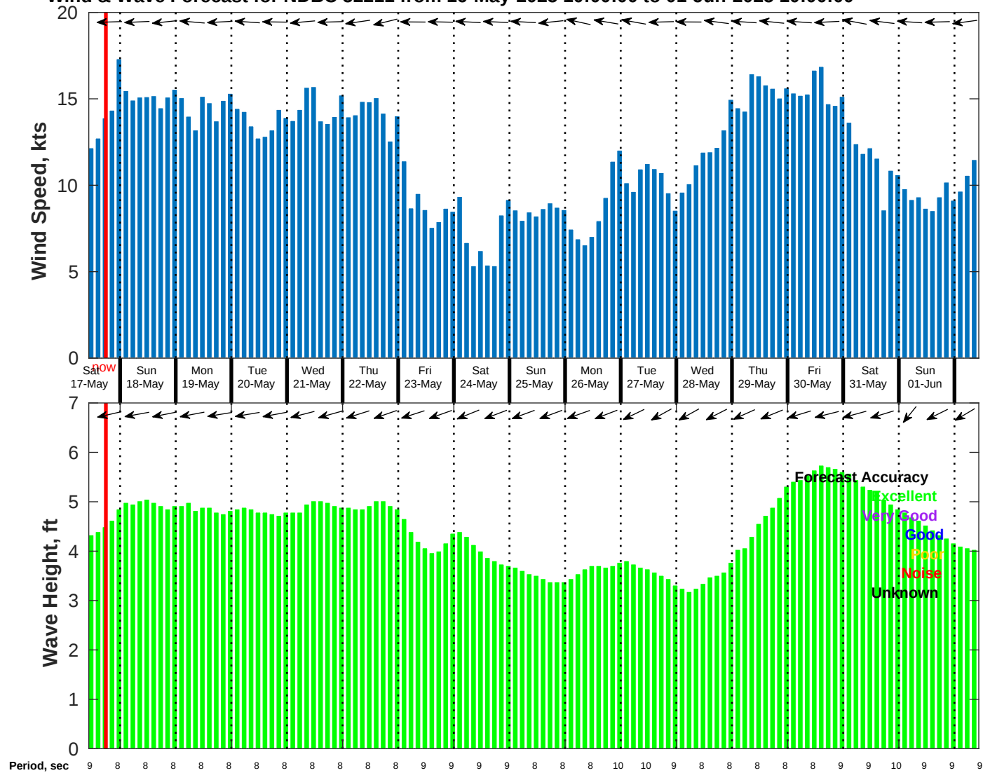
Wind & Wave Forecast for NDBC 52211 from 16-May-2025 10:00:00 to 01-Jun-2025 10:00:00
