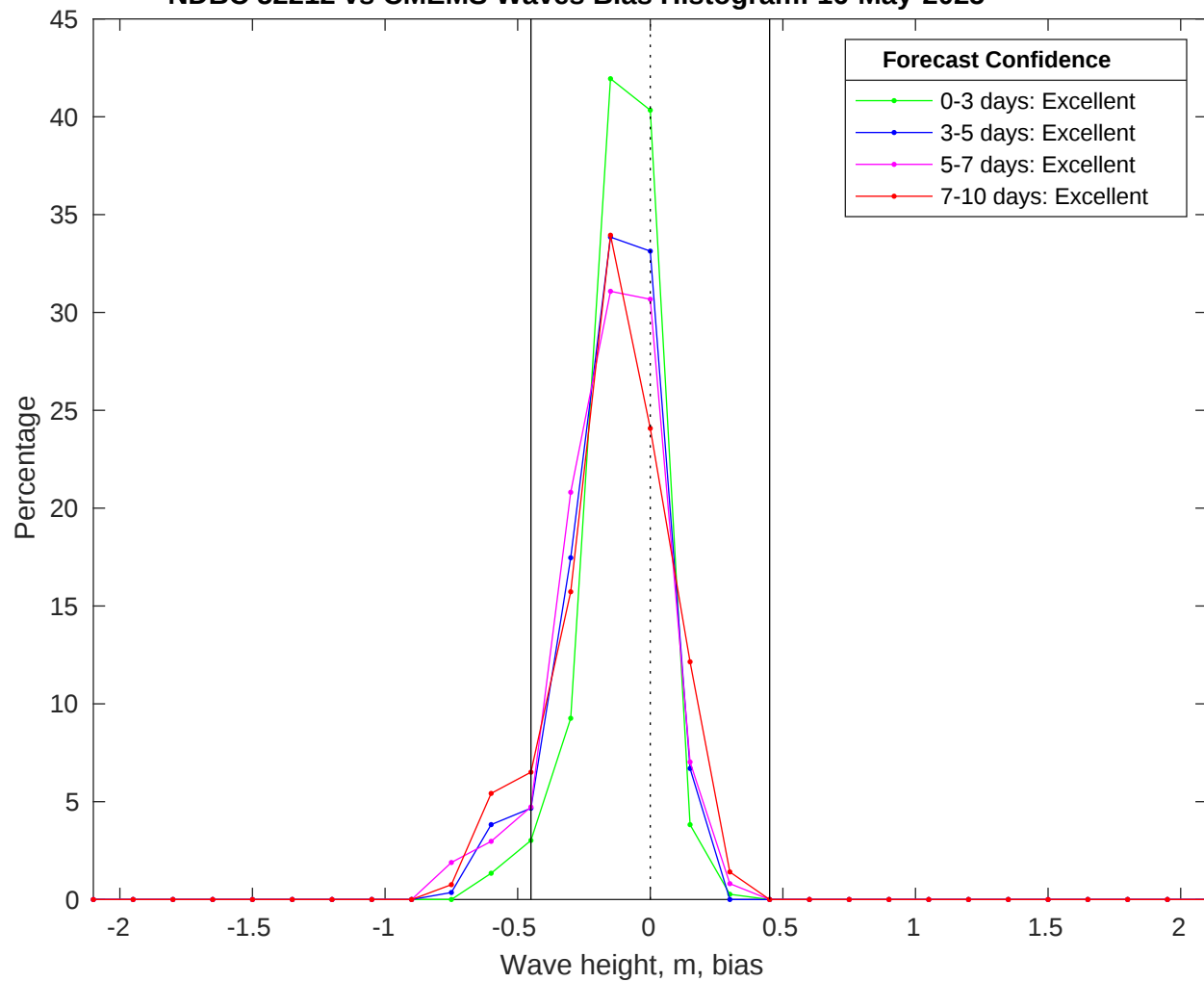
NDBC 52212 vs CMEMS Waves Bias Histogram: 16-May-2025
