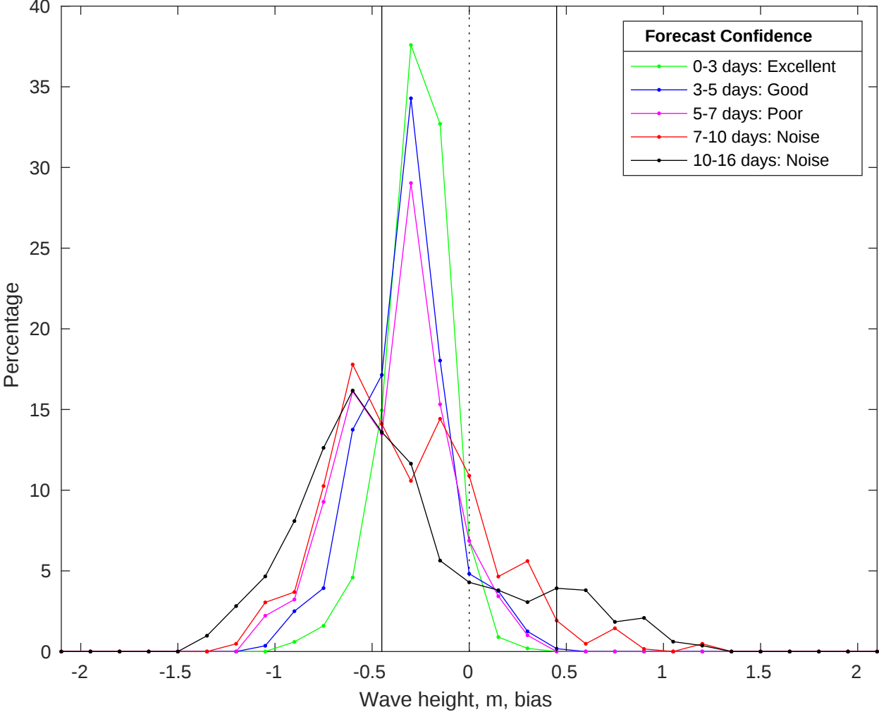
NDBC 52212 vs GFS Waves Bias Histogram: 16-May-2025
