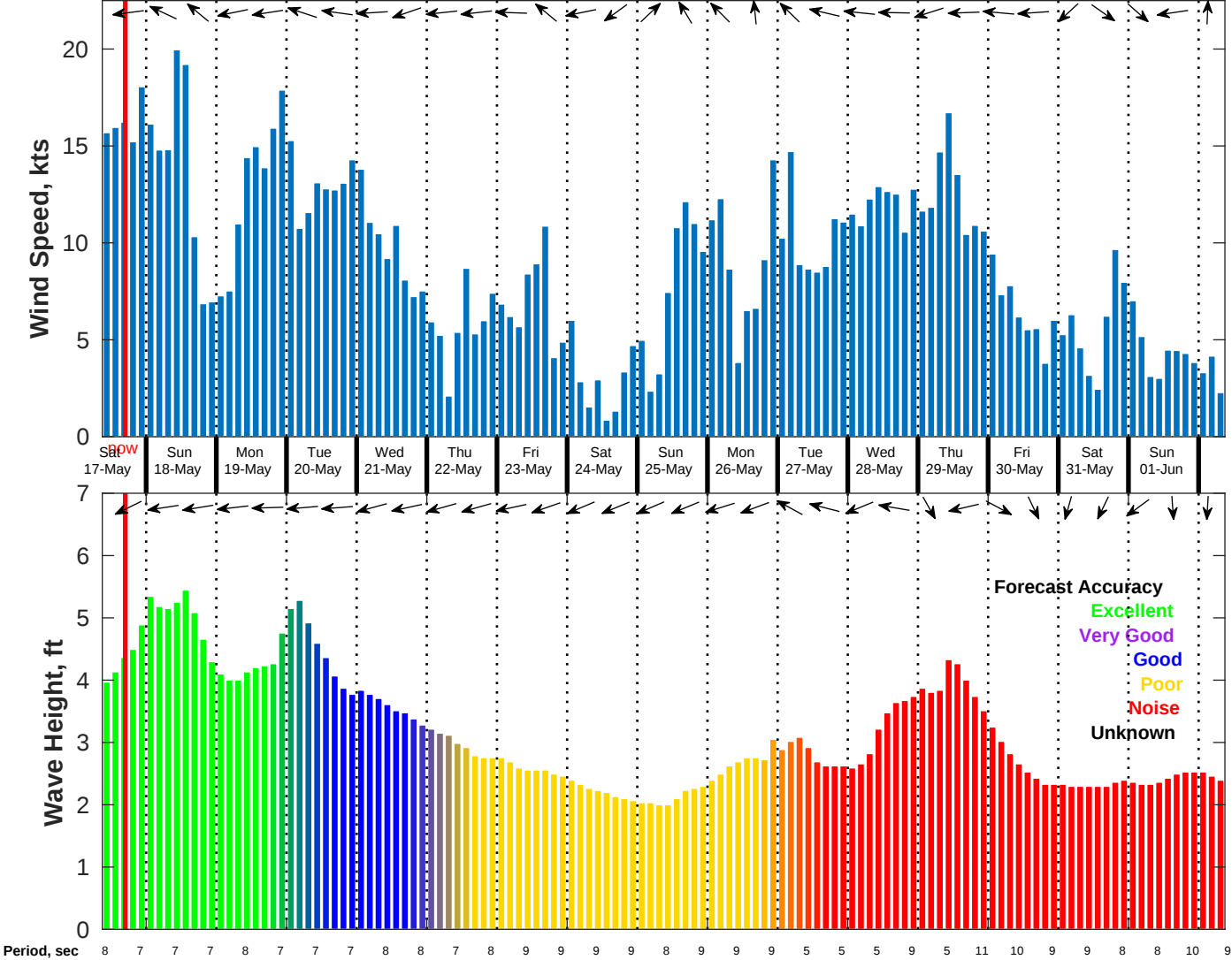
Wind & Wave Forecast for NDBC 52212 from 16-May-2025 09:00:00 to 01-Jun-2025 09:00:00
