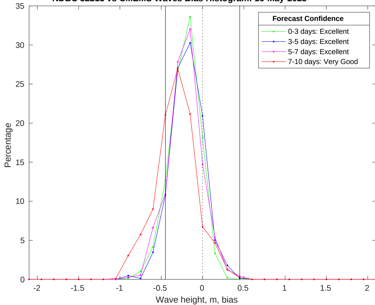
NDBC 52213 vs CMEMS Waves Bias Histogram: 16-May-2025
