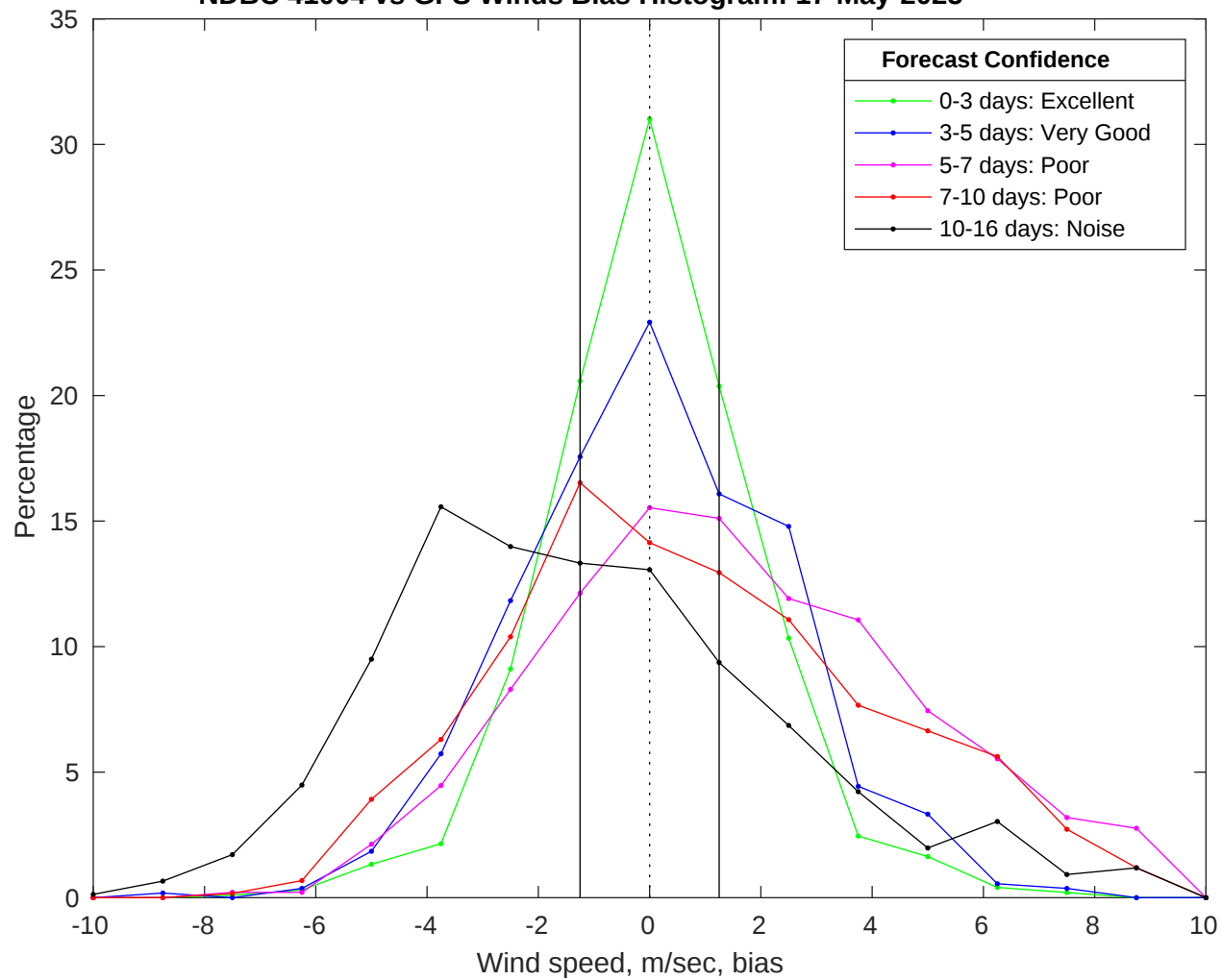
NDBC 41004 vs GFS Winds Bias Histogram: 17-May-2025
