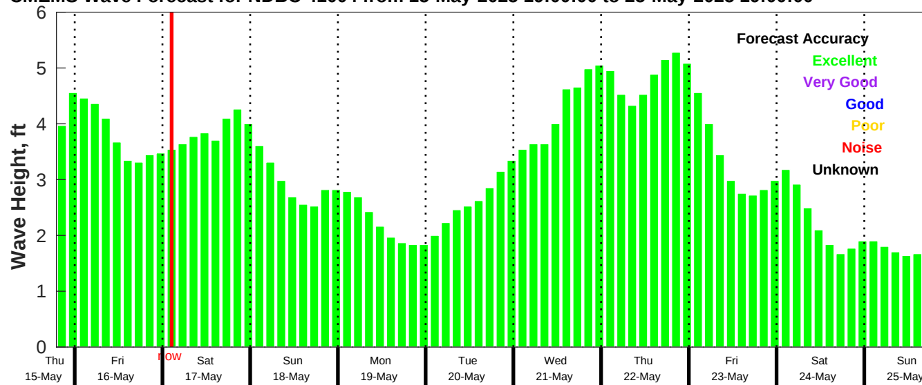
CMEMS Wave Forecast for NDBC 41004 from 15-May-2025 19:00:00 to 25-May-2025 19:00:00
