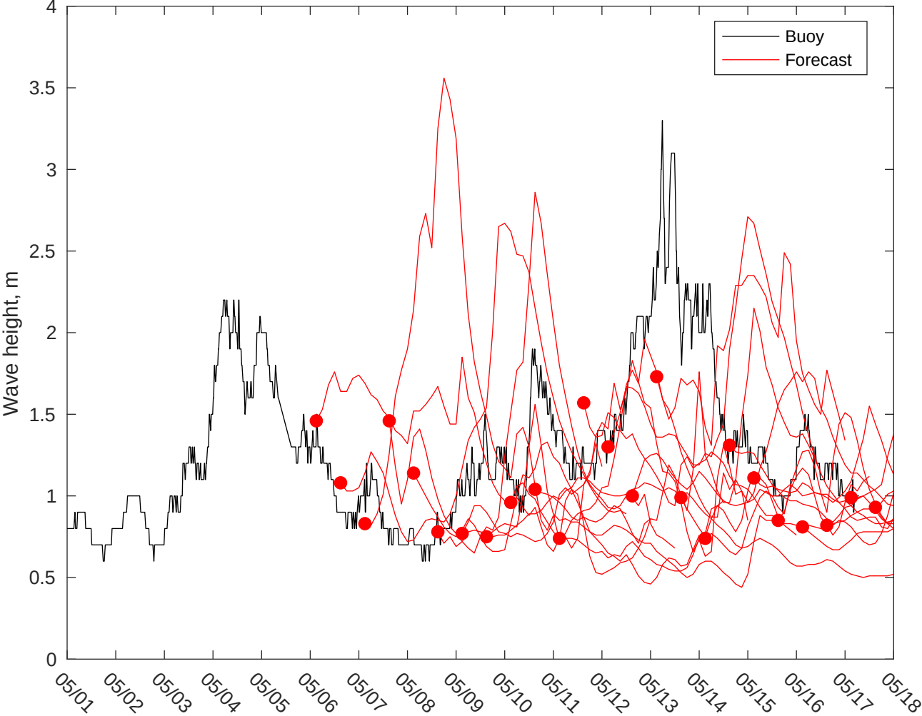
NDBC 41013 vs GFS Waves: 10 to 16 day forecast
