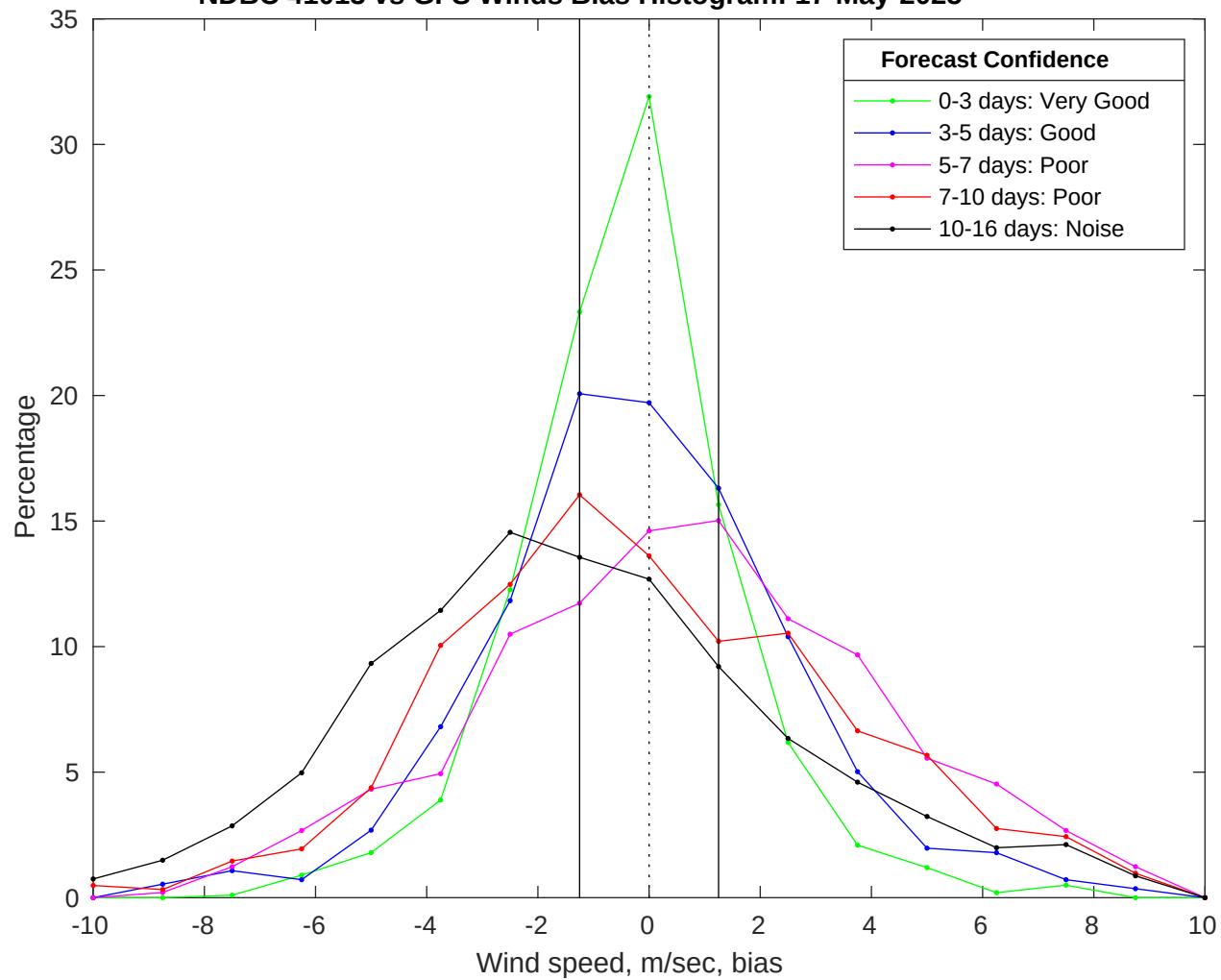
NDBC 41013 vs GFS Winds Bias Histogram: 17-May-2025
