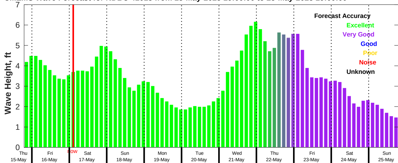
CMEMS Wave Forecast for NDBC 41013 from 15-May-2025 19:00:00 to 25-May-2025 19:00:00
