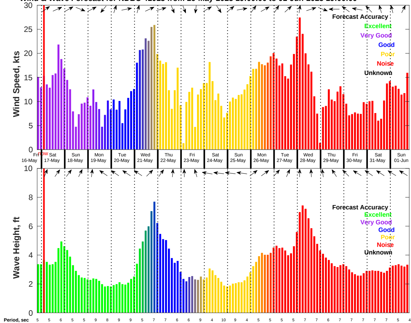
Wind & Wave Forecast for NDBC 41013 from 16-May-2025 19:00:00 to 01-Jun-2025 19:00:00
