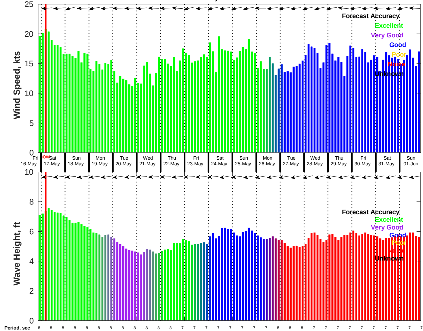
Wind & Wave Forecast for NDBC 41040 from 16-May-2025 21:00:00 to 01-Jun-2025 21:00:00
